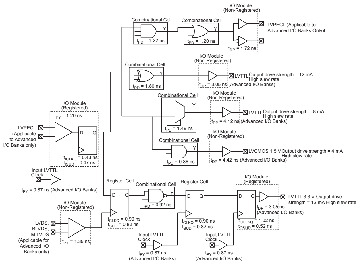
Figure 2-3 • Timing Model
