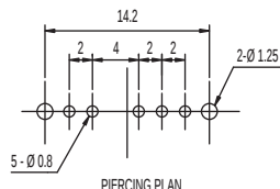
PIERCING PLAN
