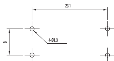
PIERCING PLAN
