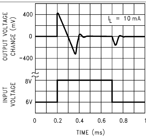
Figure 10. Line Transient Response
