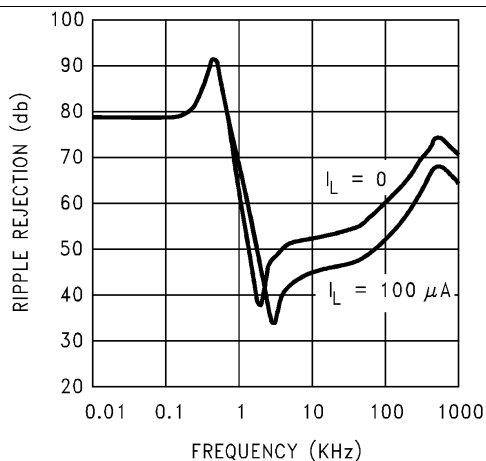
Figure 9. Ripple Rejection
