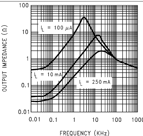
Figure 12. Output Impedance
