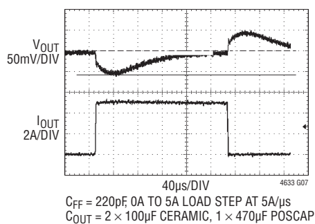
12V to 1.8V Load Step Response
