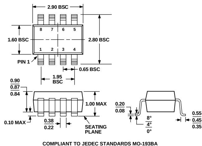
Figure 36. 8-Lead Thin Small Outline Transistor Package [TSOT] (UJ-8)
