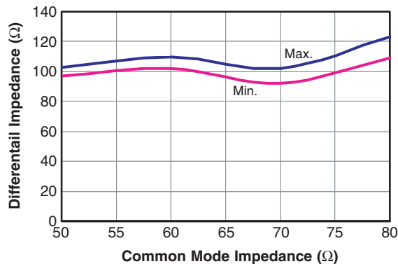
Figure 8. Differential Impedance
