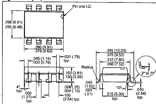
Figure 5. 8-pln SOP (PCMCIA)
