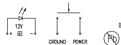
INTERNAL CIRCUIT
