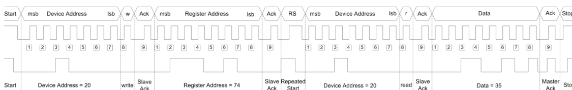
Figure 17: Read Cycle Diagram
