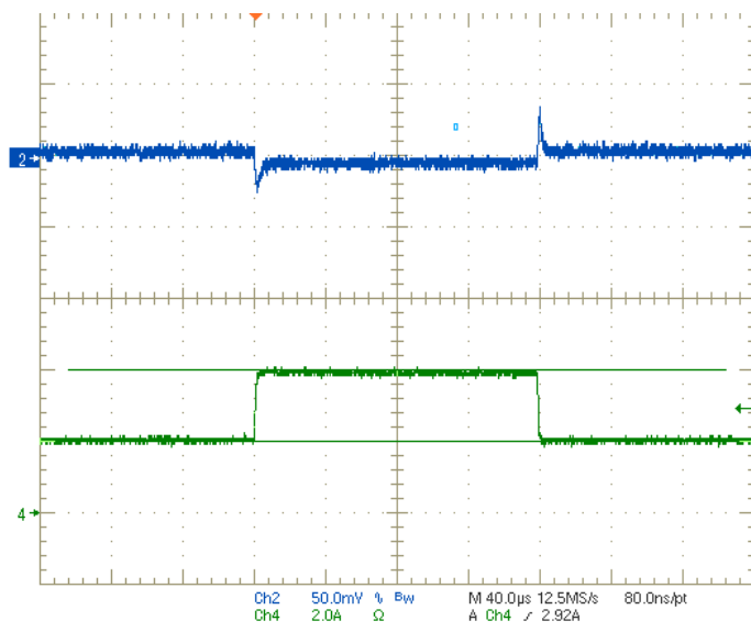
Figure 5. Step Response
