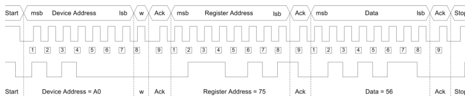
Figure 16: Write Cycle Diagram
