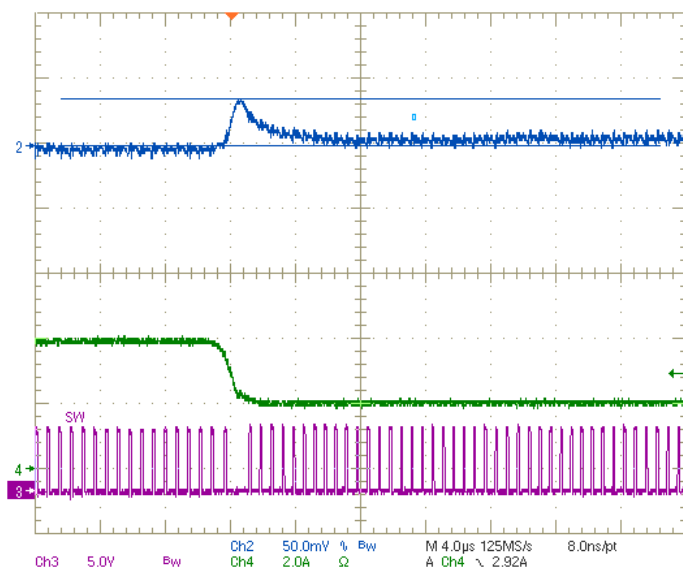
Figure 7. Step Response Falling Edge
