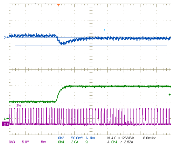
Figure 6. Step Response Rising Edge
