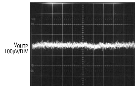
OUTP 10Hz to 100kHz Output Noise C_{BYP} = 0.01\mu F
