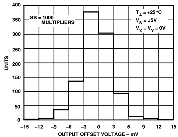
Figure 36. Output Offset Voltage ( Z_{OS} ) Distribution
