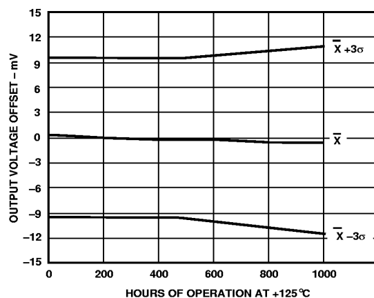
Figure 41. Output Voltage Offset ( Z_{OS} ) Distribution Accelerated by Burn-in
