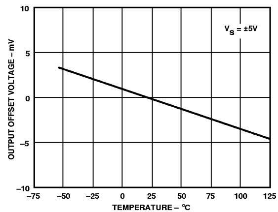
Figure 37. Output Offset Voltage ( Z_{OS} ) vs. Temperature
