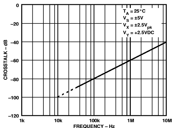
Figure 20. Crosstalk vs. Frequency
