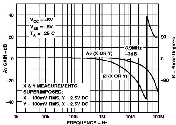
Figure 1. Gain & Phase vs. Frequency Response
