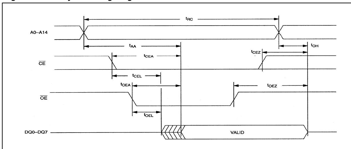
Figure 5. Read Cycle Timing Diagram
