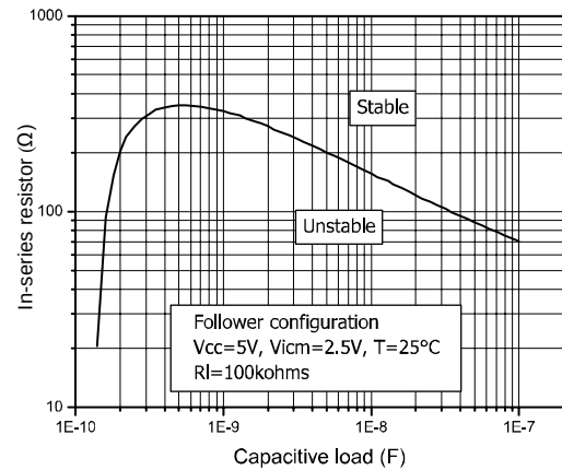
Figure 3: In-series resistor ( R_{iso} ) vs. capacitive load
