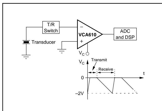
FIGURE 5. Typical Ultrasound Application.
