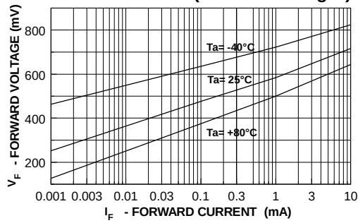
Forward Voltage vs Ambient Temperature VF - 1.0 \mu\text{A} - 10 mA (-40 to +80 Deg C)
