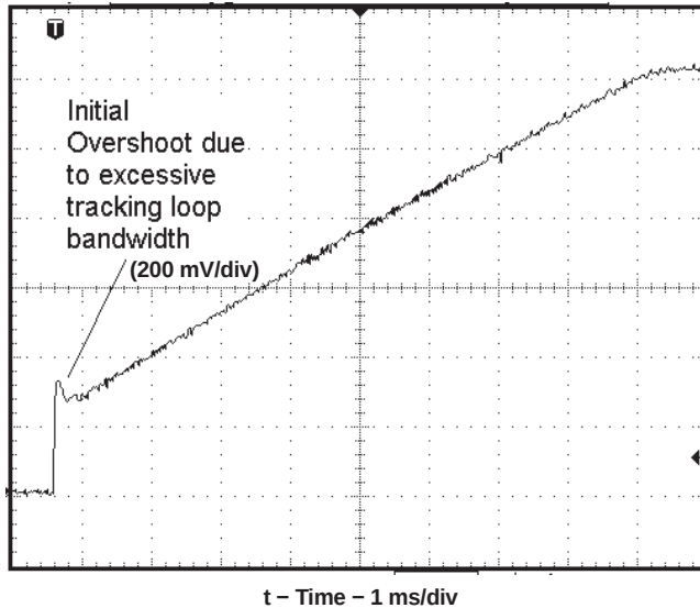
Figure 32. Excessive Tracking Loop Bandwidth
