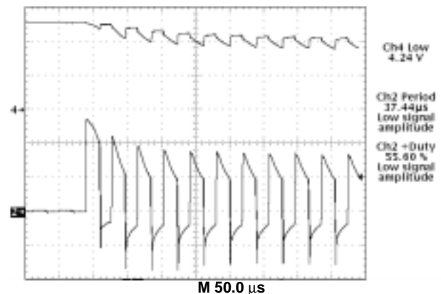
Figure 12. CS5151H Demonstration Board Hiccup Mode Short Circuit Protection. Gate Pulses are Delivered While the Soft Start Capacitor Charges, and Cease During Discharge
