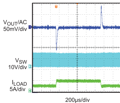
Load Transient Response I_{OUT}=2.25A to 4.5A , Step @ 1A/\mu s
