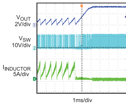
Hiccup with Output Short Recovery
