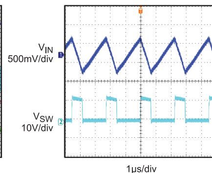
Input Ripple Voltage I_{OUT}=10A
