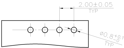
RECOMMENDER PCB LAYOUT (PCB THK=1.0~1.6mm)
