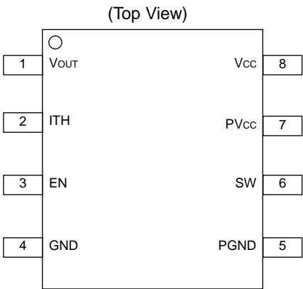
Figure 2. Pin Configuration
