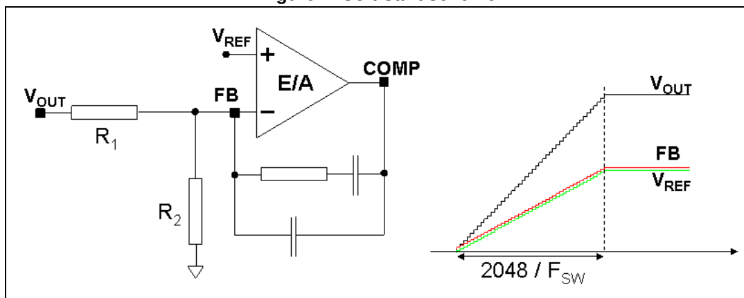
Figure 7. Soft-start scheme
