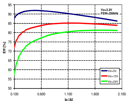
Figure 27. Efficiency vs. output current at V_O = 3.3\text{ V}
