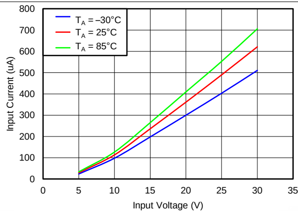
Figure 2. Input Supply Current vs Supply Voltage
