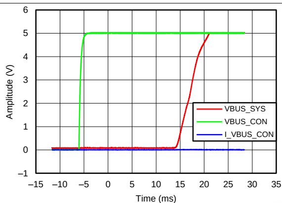
Figure 8. Power Up With 2.2 \mu F on V_{BUS\_SYS}
