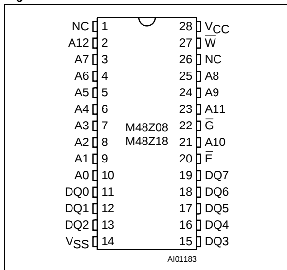
Figure 3. DIP Connections
