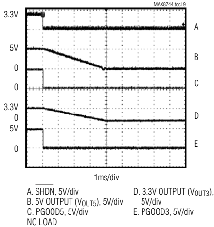
SMPS SHUTDOWN WAVEFORM
