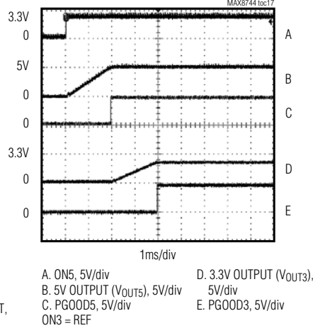
SMPS DELAYED STARTUP SEQUENCE (ON3 = REF)
