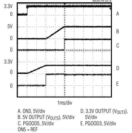
SMPS DELAYED STARTUP SEQUENCE (ON5 = REF)
