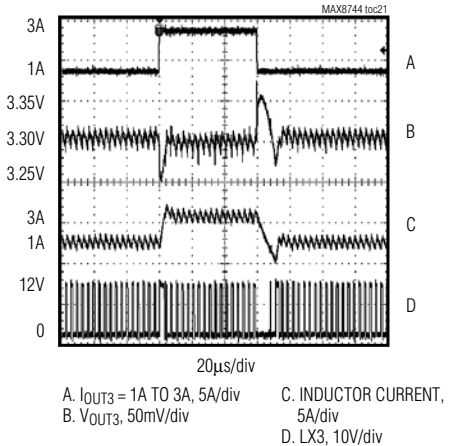
OUT3 LOAD TRANSIENT
