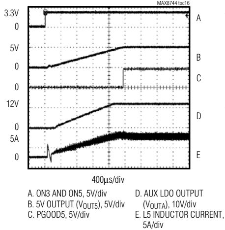
SOFT-START WAVEFORM
