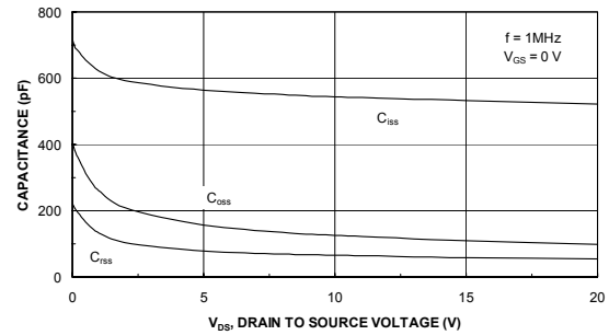
Figure 8. Capacitance Characteristics.
