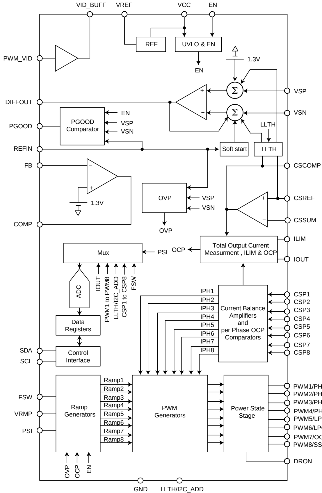
Figure 5. NCP81274 Functional Block Diagram
