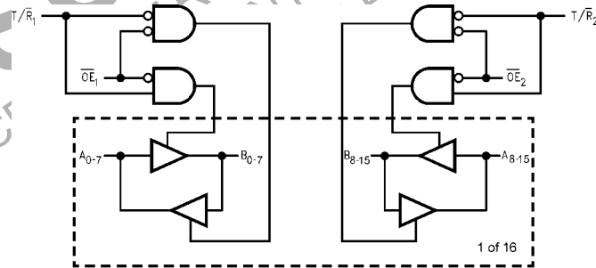
Figure 3. Logic Diagram
