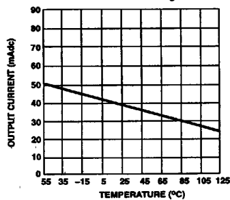
Current Limiting
