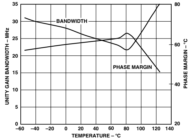
TPC 5. Unity Gain Bandwidth and Phase Margin vs. Temperature
