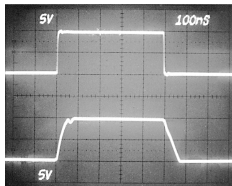
TPC 17. Noninverting Large Signal Pulse Response, R_L = 1\text{ k}\Omega
