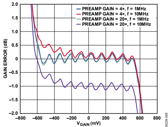
Figure 9. Gain Error vs. V_{\text{GAIN}} at 1 MHz and 10 MHz and for Preamp Gains of 4x and 20x (See Figure 56)
