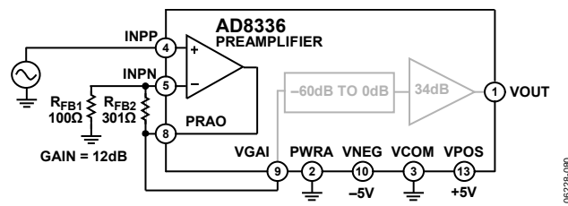
Figure 80. Circuit Configuration for Noninverting Gain
