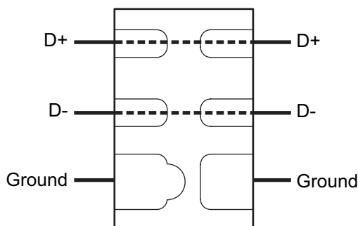
Figure 2. Flow-through Layout
