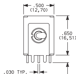
Actuator Shown In Pos. 1 .125 TYP. (3,18) Terminals & Support
