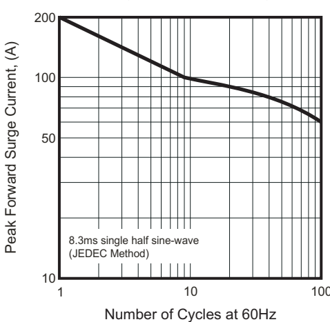
Fig.3 - Maximum Non-repetitive Forward Surge Current Per Bridge Element
