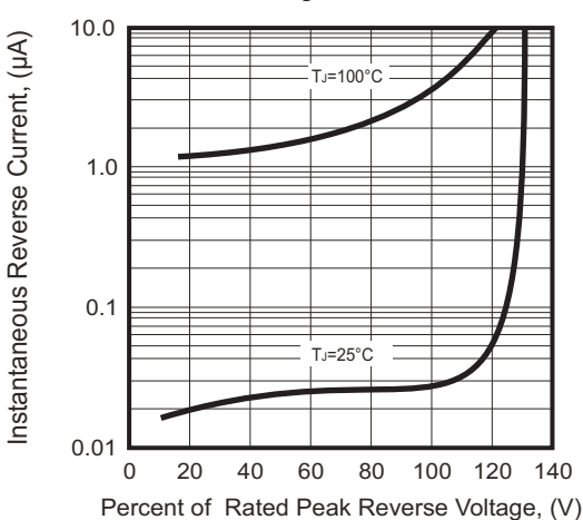
Fig.4 - Typical Reverse Characteristics Per Bridge Element
