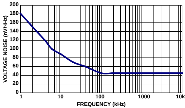
FIGURE 21. OUTPUT VOLTAGE NOISE vs FREQUENCY
