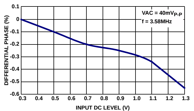
FIGURE 18. DIFFERENTIAL PHASE
