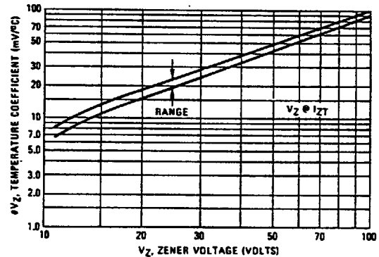
Figure 4 TEMPERATURE COEFFICIENTS
