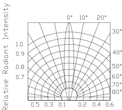
VIEW ANGLE EP2012-150XX
