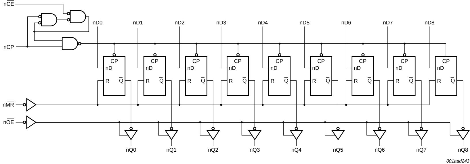
Fig 4. Logic diagram
