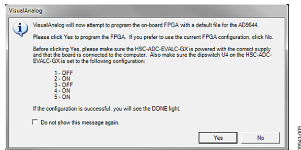
Figure 5. VisualAnalog Default Configuration Message
