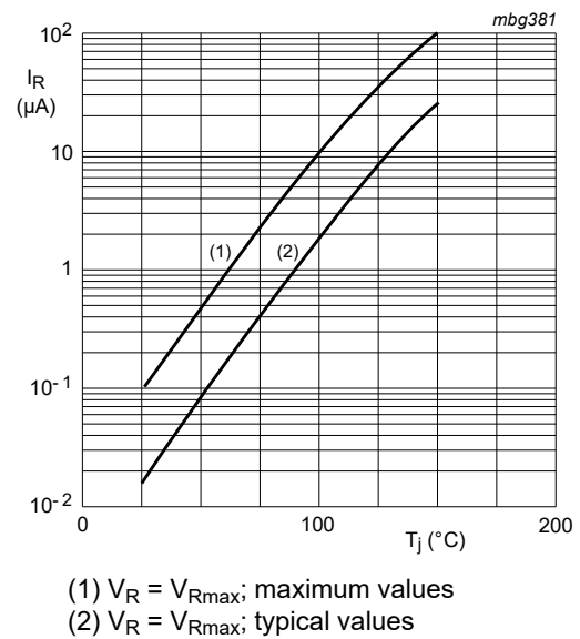
Fig. 2. Reverse current as a function of junction temperature
