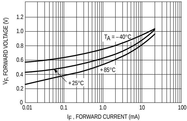
Figure 9. Forward Characteristics
