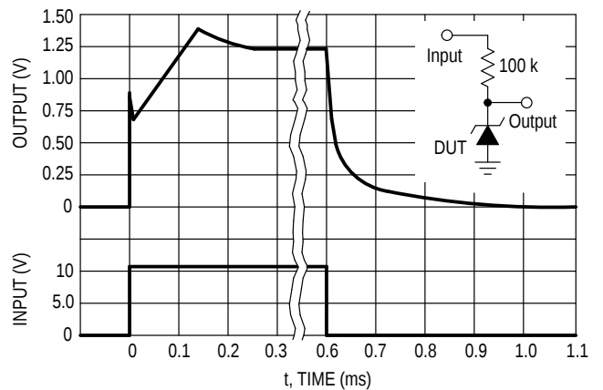
Figure 6. Response Time
