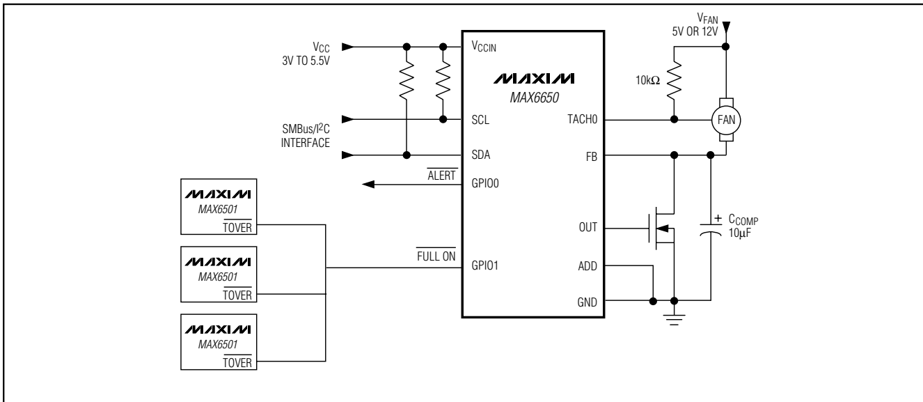
Figure 12. MAX6651 Hardware Fail-Safe
