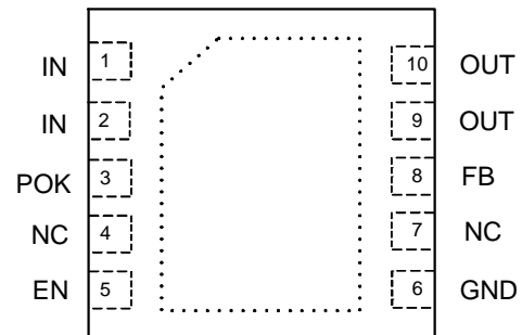
DFN3030-10
