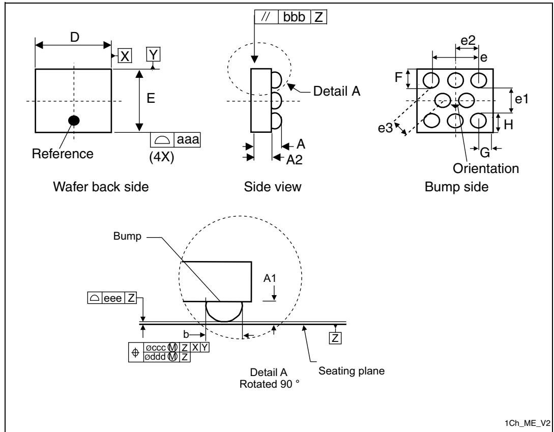
Figure 20. M24128-DFCS6TP/K, WLCSP 8-bump wafer-level chip scale package outline
