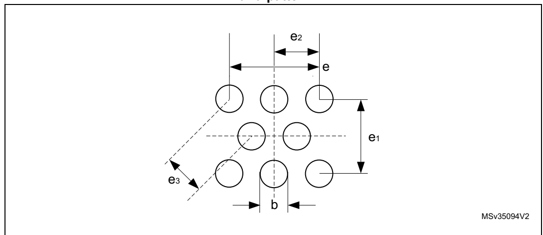
Figure 21. WLCSP 8-bump wafer-length chip-scale package recommended land pattern
