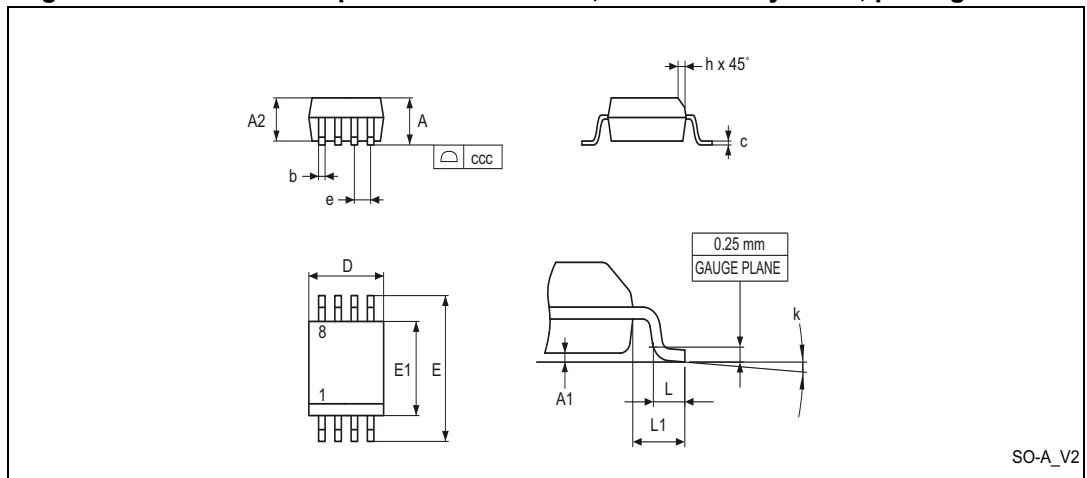
Figure 18. SO8N – 8-lead plastic small outline, 150 mils body width, package outline
