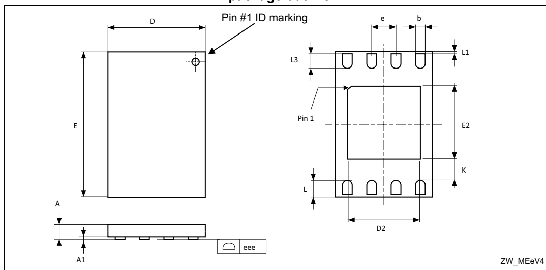
Figure 19. UFDFPN8 (MLP8) – 8-lead ultra thin fine pitch dual flat no lead, package outline
