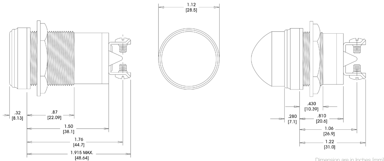
Dimension are in Inches [mm]
