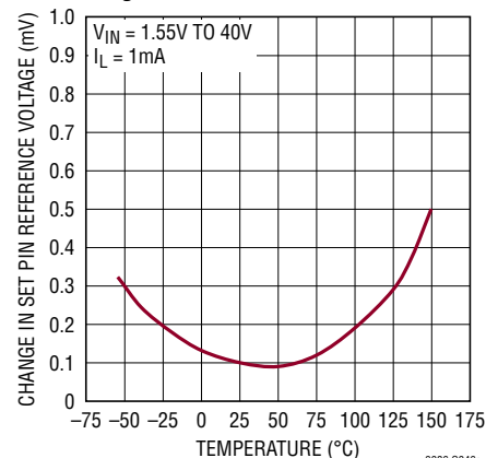
Reference Voltage Line Regulation
