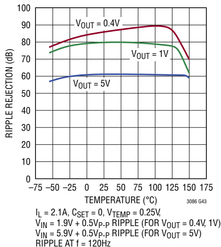
Ripple Rejection vs Temperature
