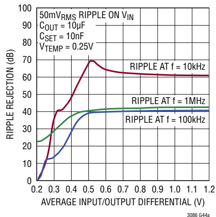
5V, 1A Ripple Rejection vs V_{IN} - V_{OUT}
