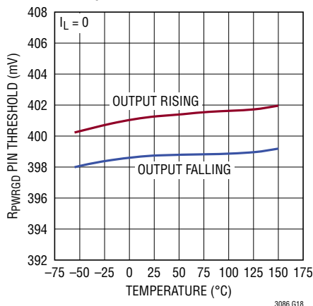
RpWRGD Pin Threshold
