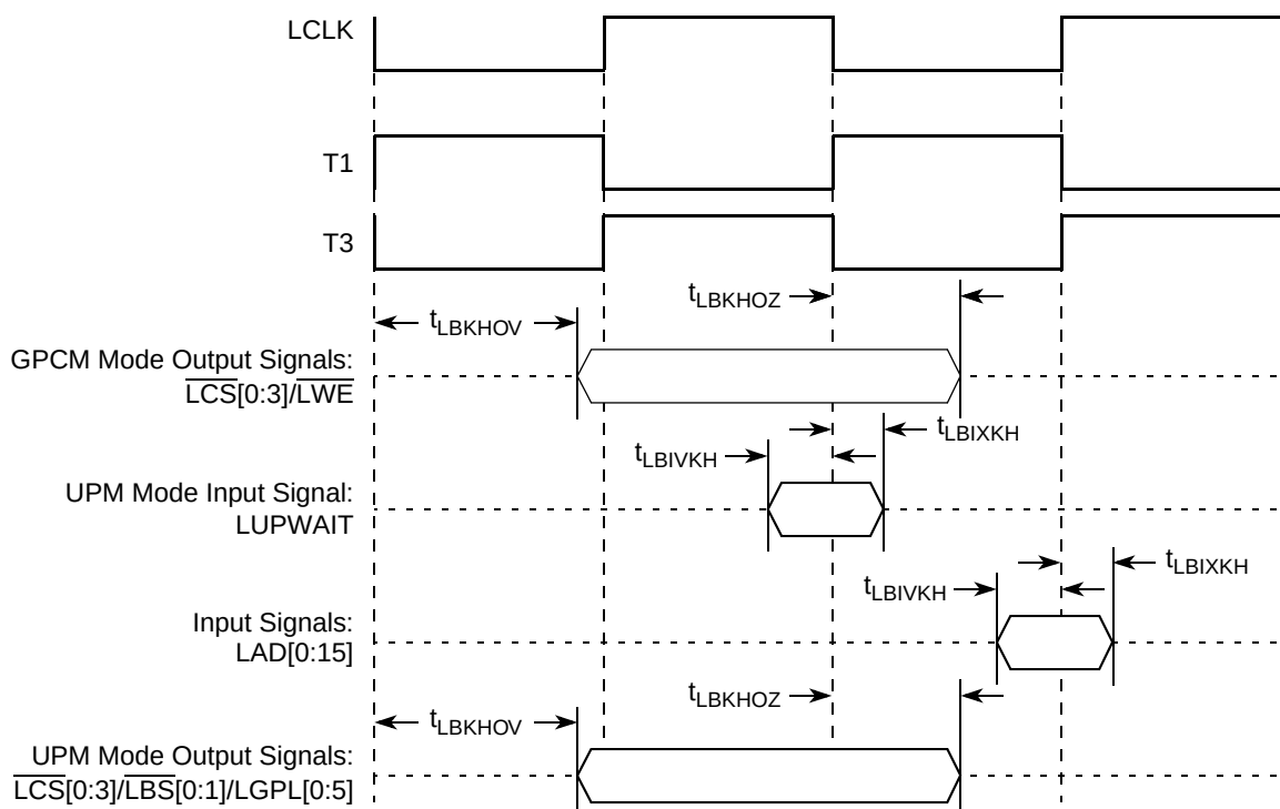
Figure 38. Local Bus Signals, GPCM/UPM Signals for LCRR[CLKDIV] = 2
