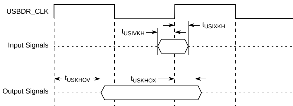
Figure 35. USB Signals
