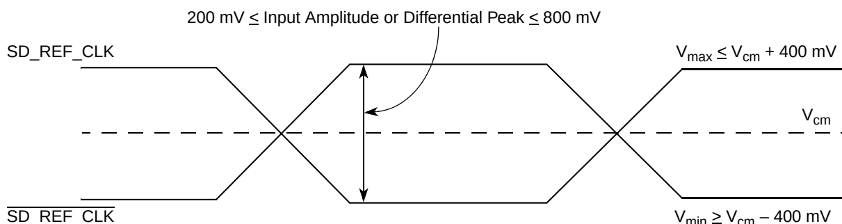
Figure 25. Differential Reference Clock Input DC Requirements (External AC-Coupled)
