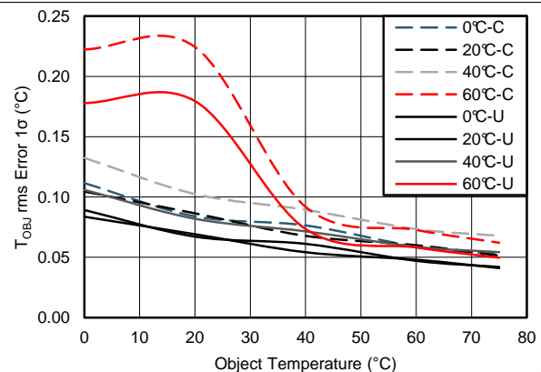
Figure 51. Noise in Temperature Measurement, Wide Range Over T_{\text{DIE}}
