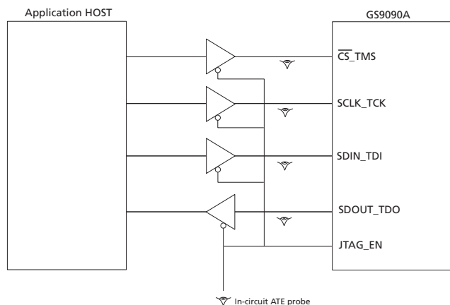
Figure 3-21: In-Circuit JTAG
