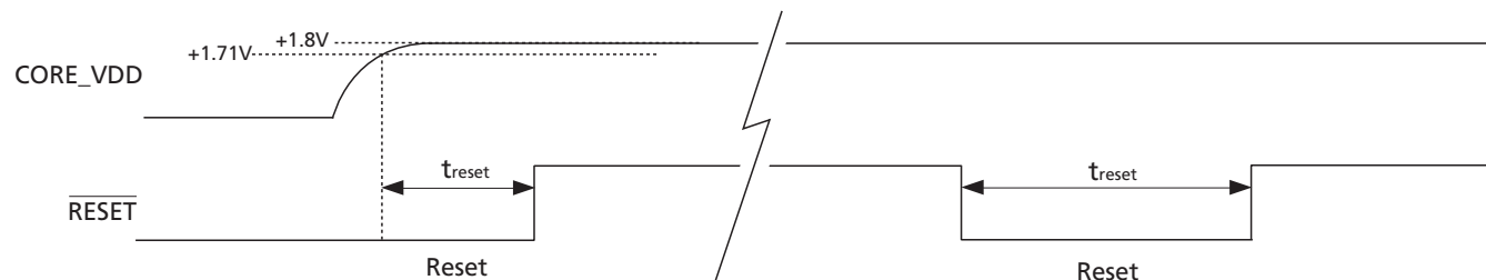
Figure 3-23: Reset pulse
