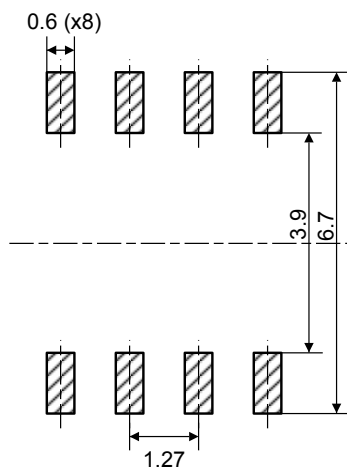
Figure 20. SO8N - Recommended footprint
