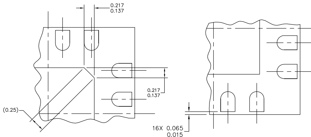
DETAIL M PIN 1 BACKSIDE IDENTIFIER
